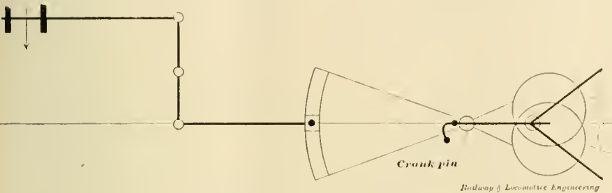
INSIDE ADMISSION-INDIRECT.
